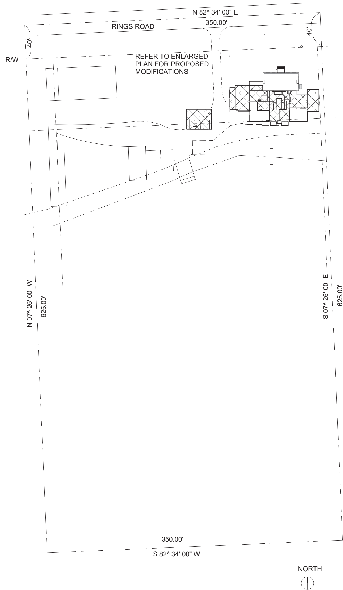
② Overall Site Plan 1" = 60'-0"
