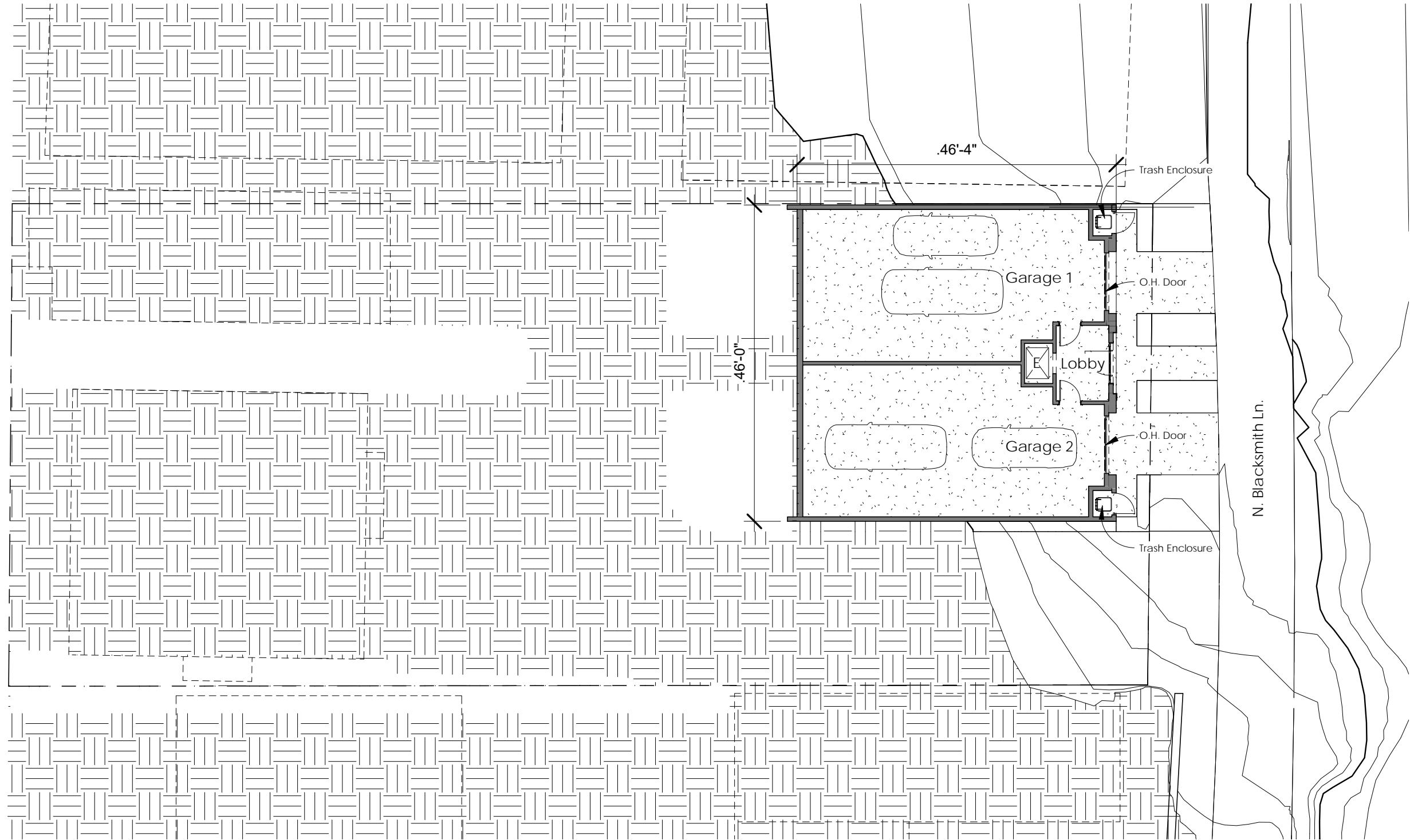
① Garage/Storage Level 1/16" = 1'-0"
