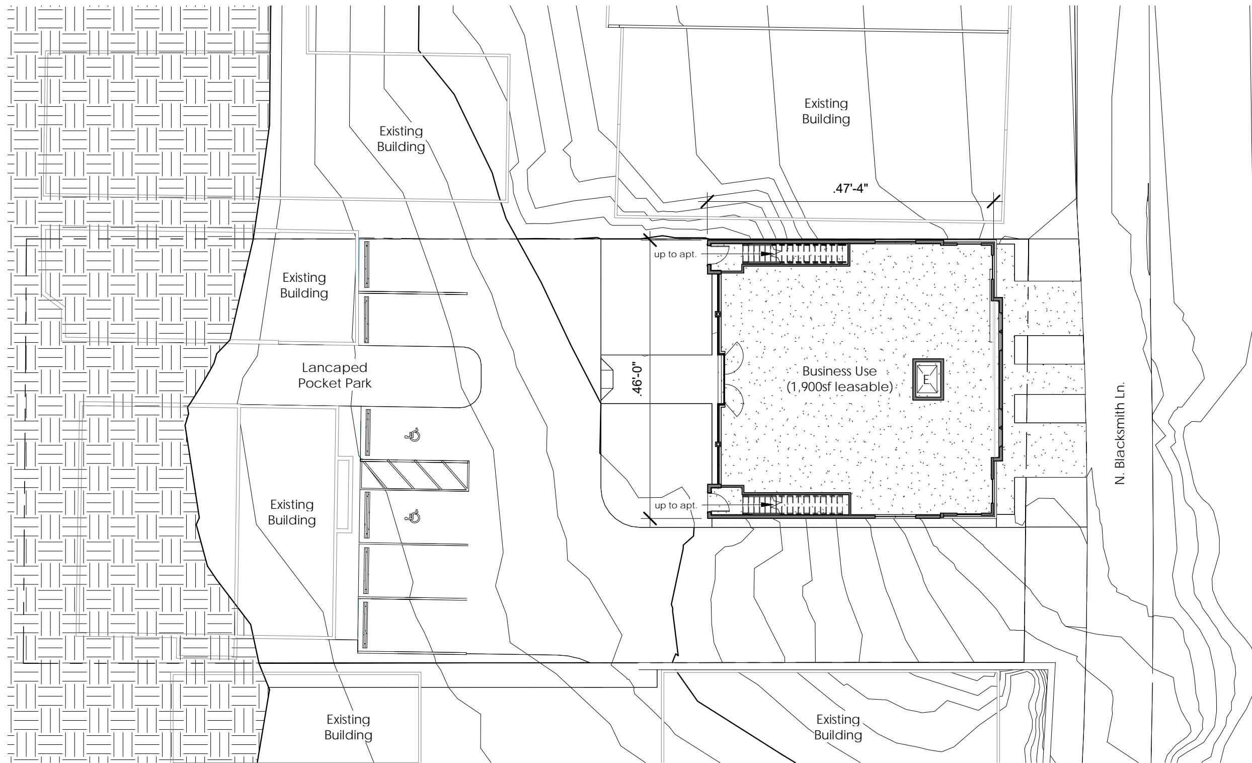
① Office Level 1/16" = 1'-0"
