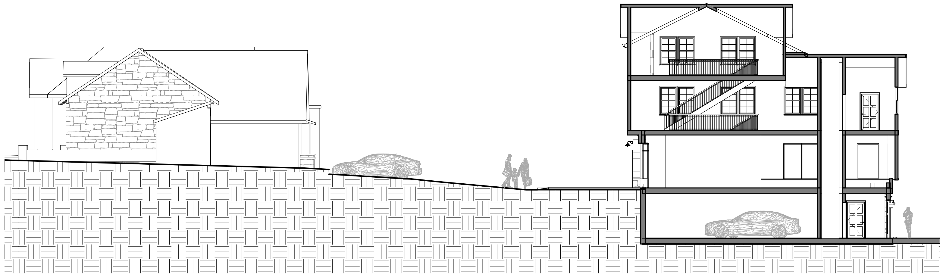
① Building Section A 3/32" = 1'-0"
