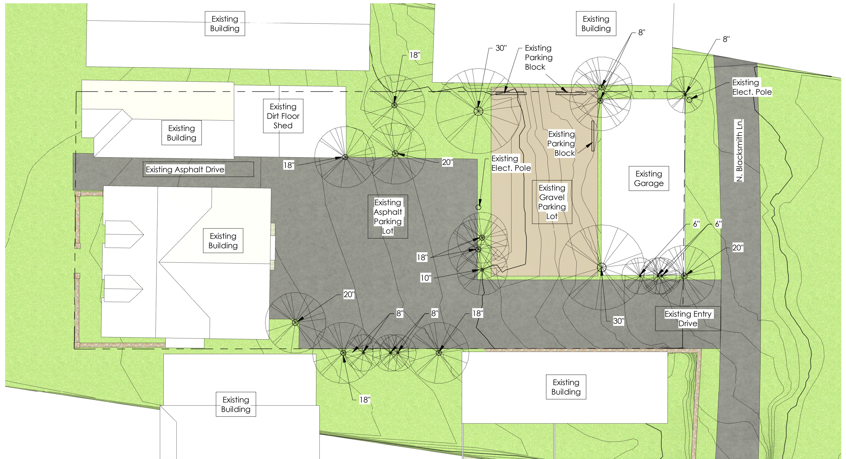
1 Site Plan - Existing Conditions 1/16" = 1'-0"
