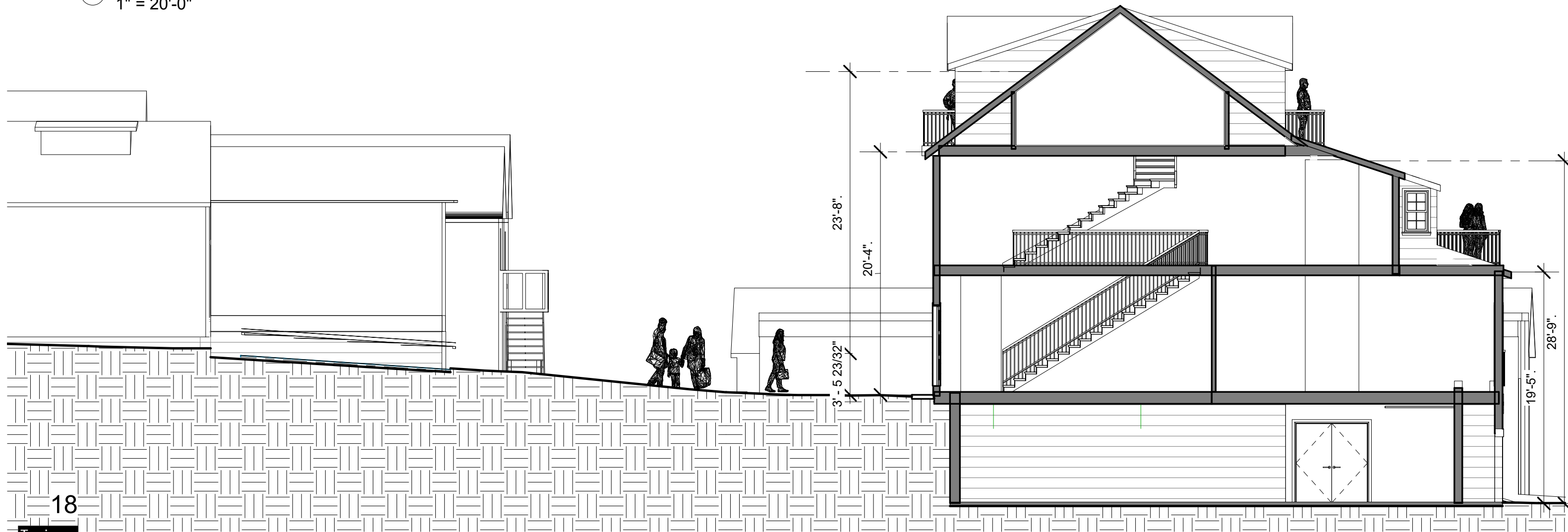
2 Building Section 1/8" = 1'-0"
