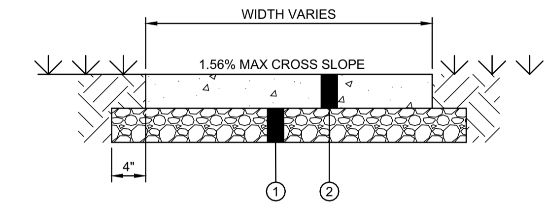
SIDEWALK SECTION NO SCALE
