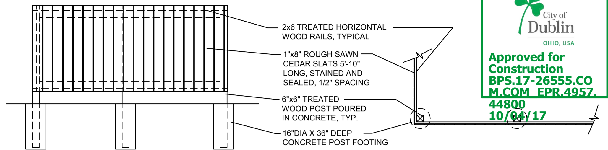
SCREENING FENCE DETAIL NO SCALE
