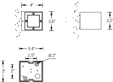
Mounting Detail
