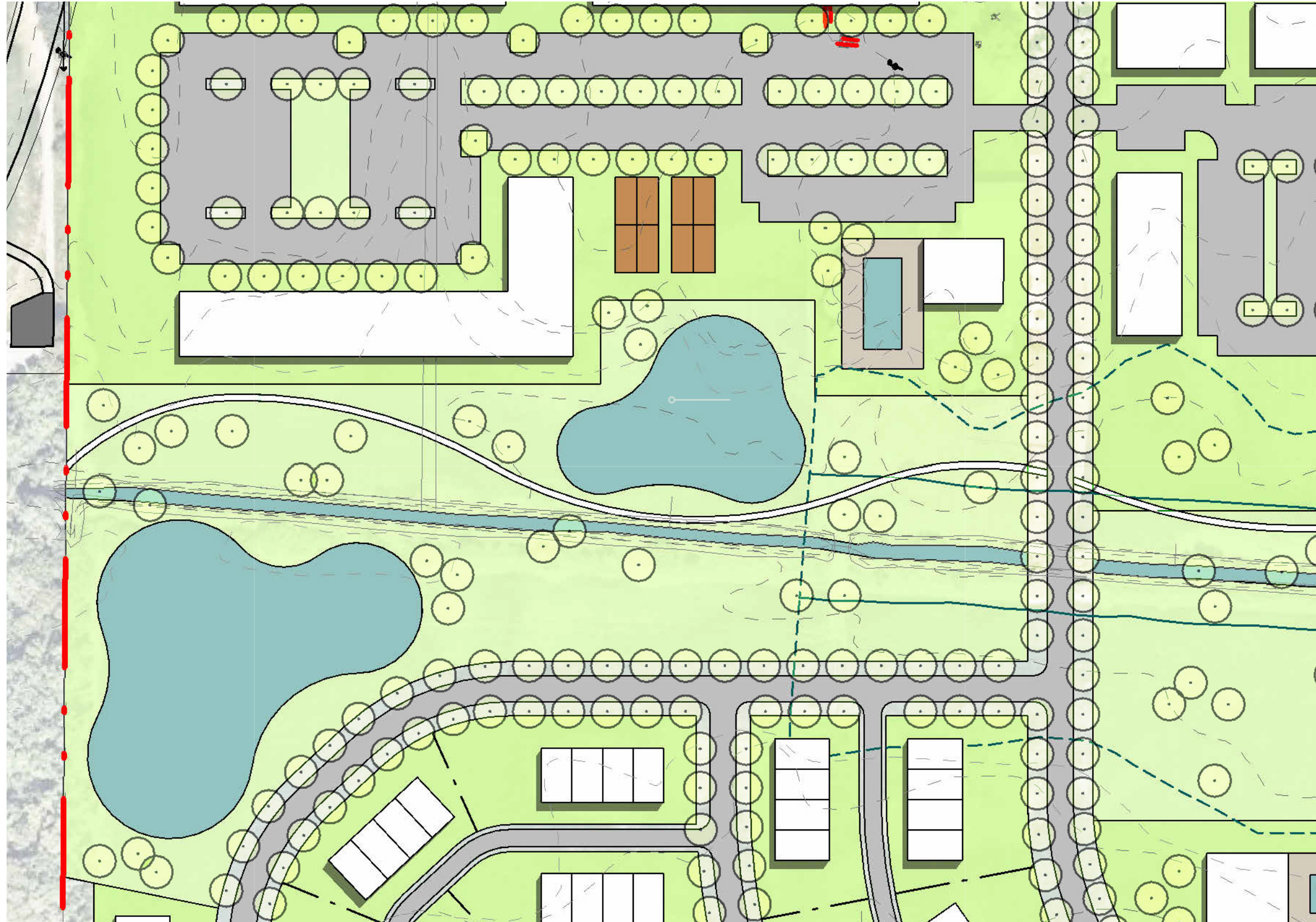
DETENTION PONDS
