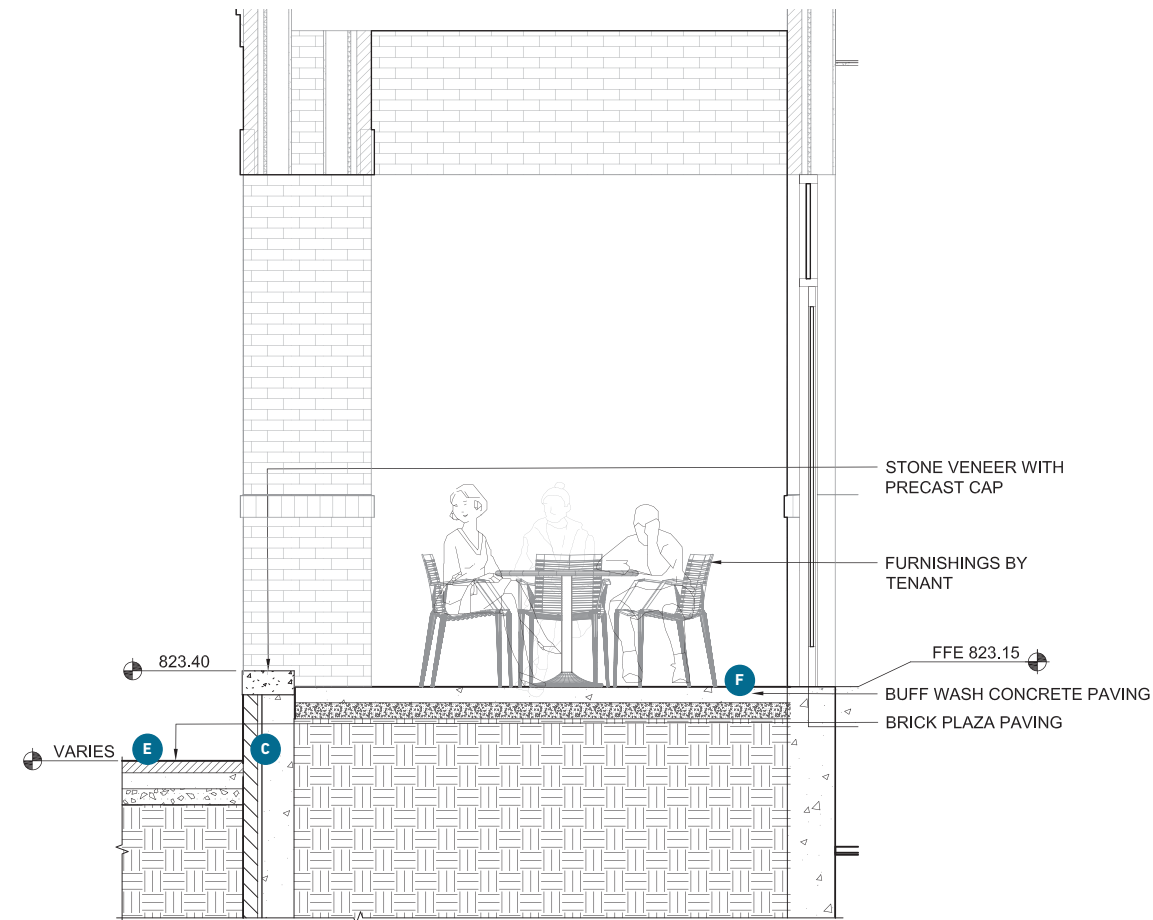
2 NORTH DINING TERRACE TYPICAL SECTION
