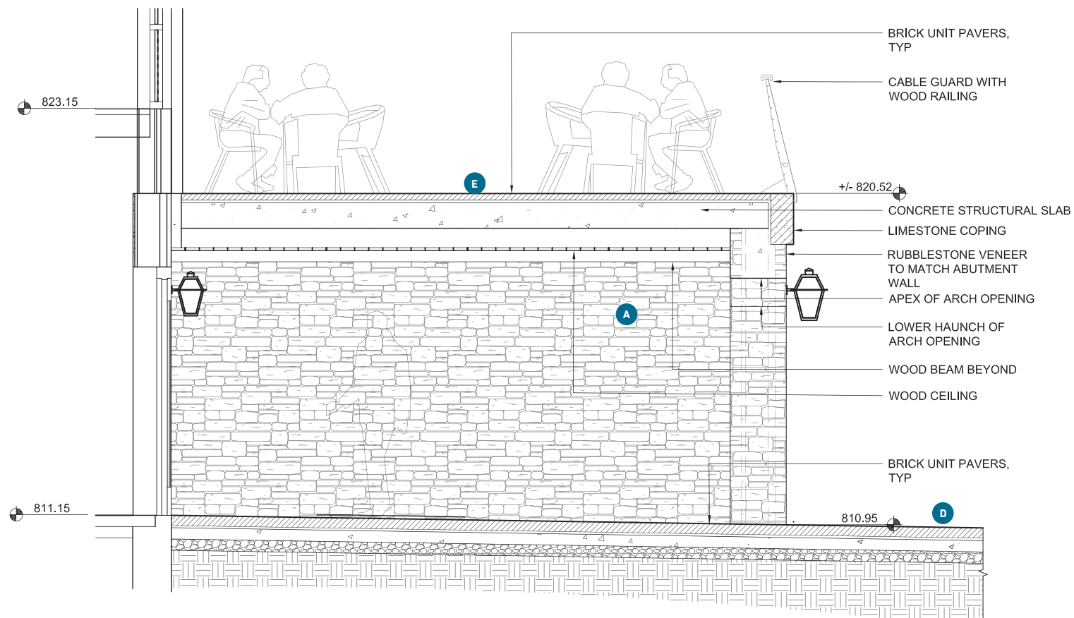
1 SPEAKEASY GROTTO BEAM TYPICAL SECTION
