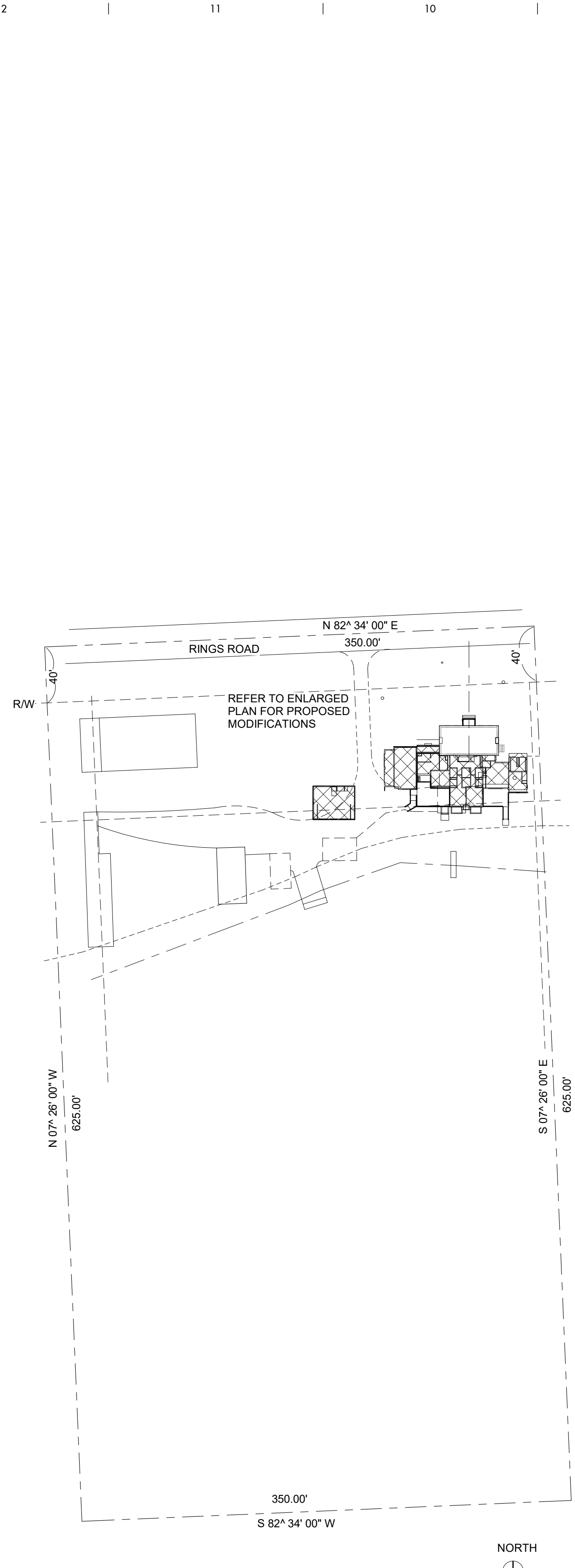
② Overall Site Plan 1" = 60'-0"
