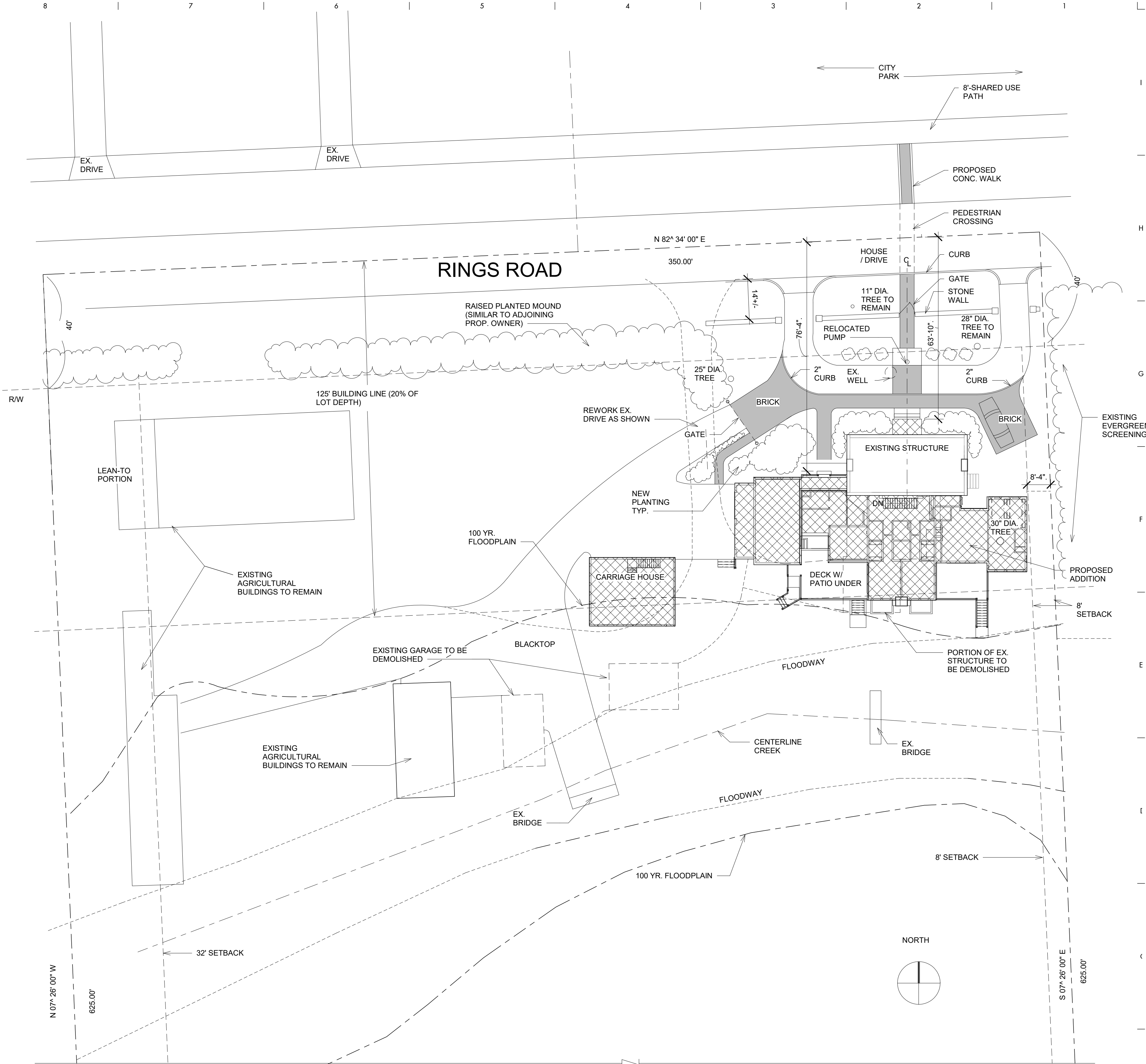
① Site Plan 1" = 20'-0"
