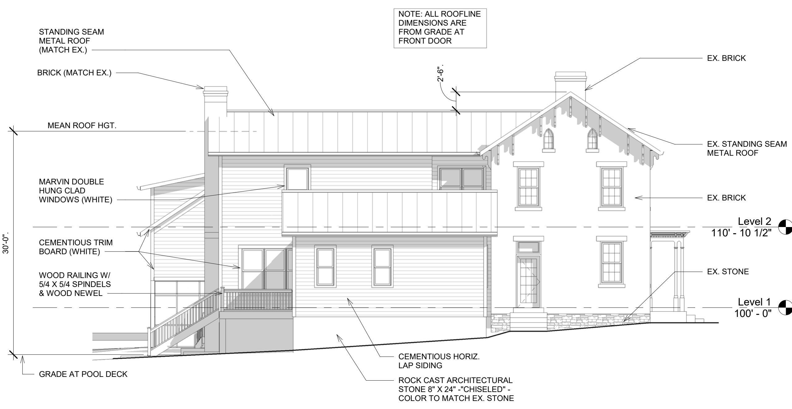
② Left Side Elevation 1/8" = 1'-0"
