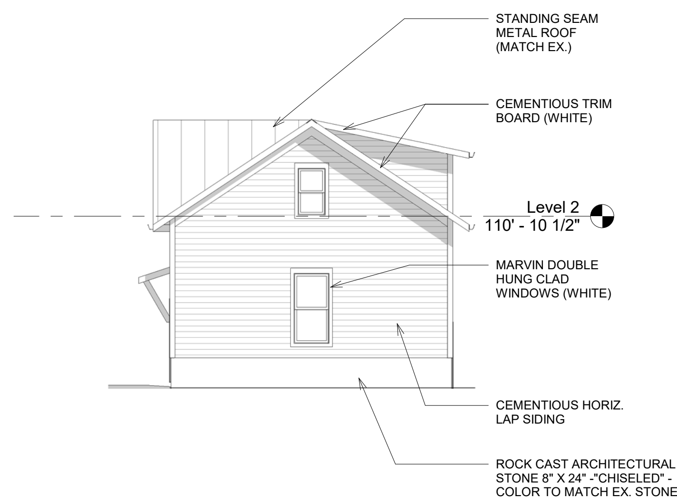
5 Right Side Elevation 1/8" = 1'-0"
