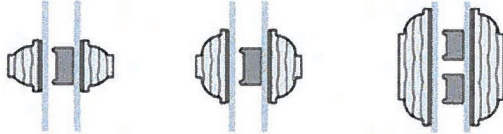
Ogee Grilles Wood Exterior, Wood Interior 7/8", 1 1/4", and 2" widths
