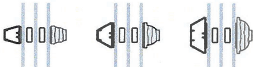
Putty Glaze and Ogee Grilles Clad Exterior, Wood Interior 5/8", 7/8", and 1 1/4" widths Triple- Pane Glass
