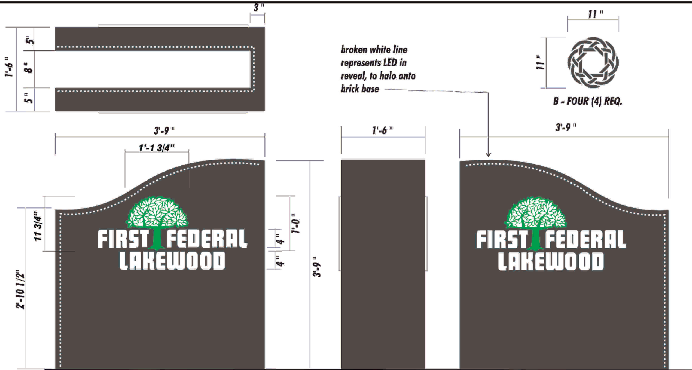
A - FACE ELEVATIONS - TWO (2) REQUIRED
