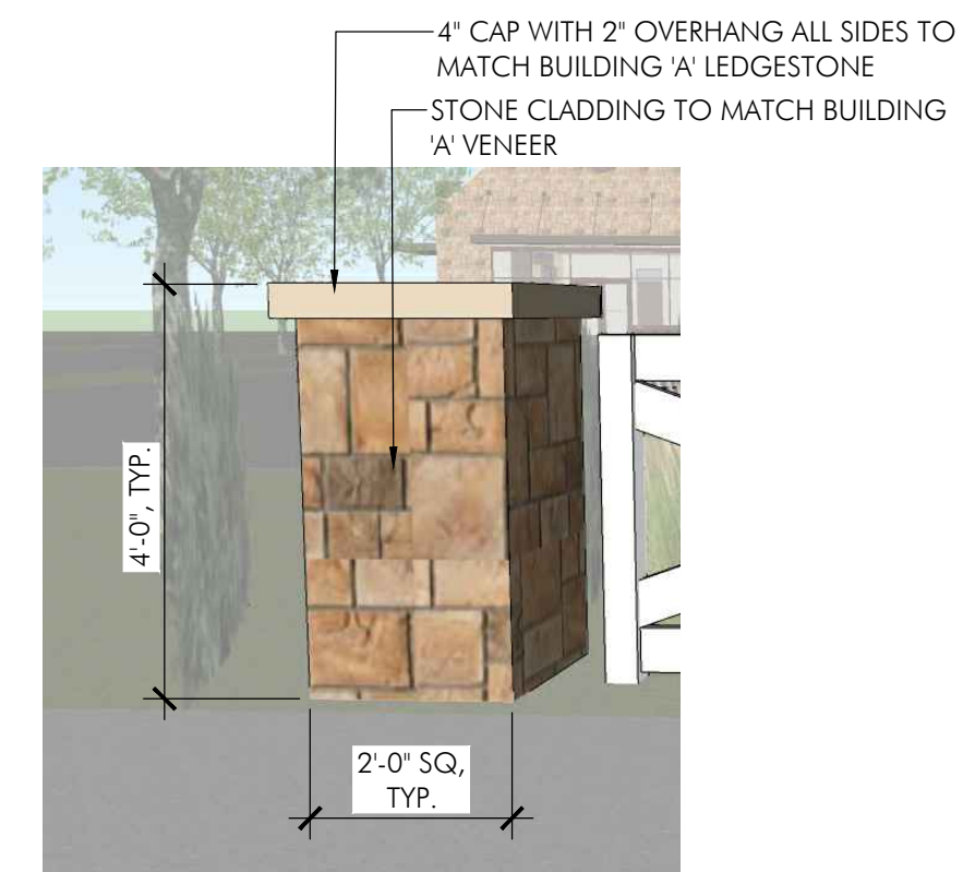
Typical Stone Column 1/2" = 1'-0"
