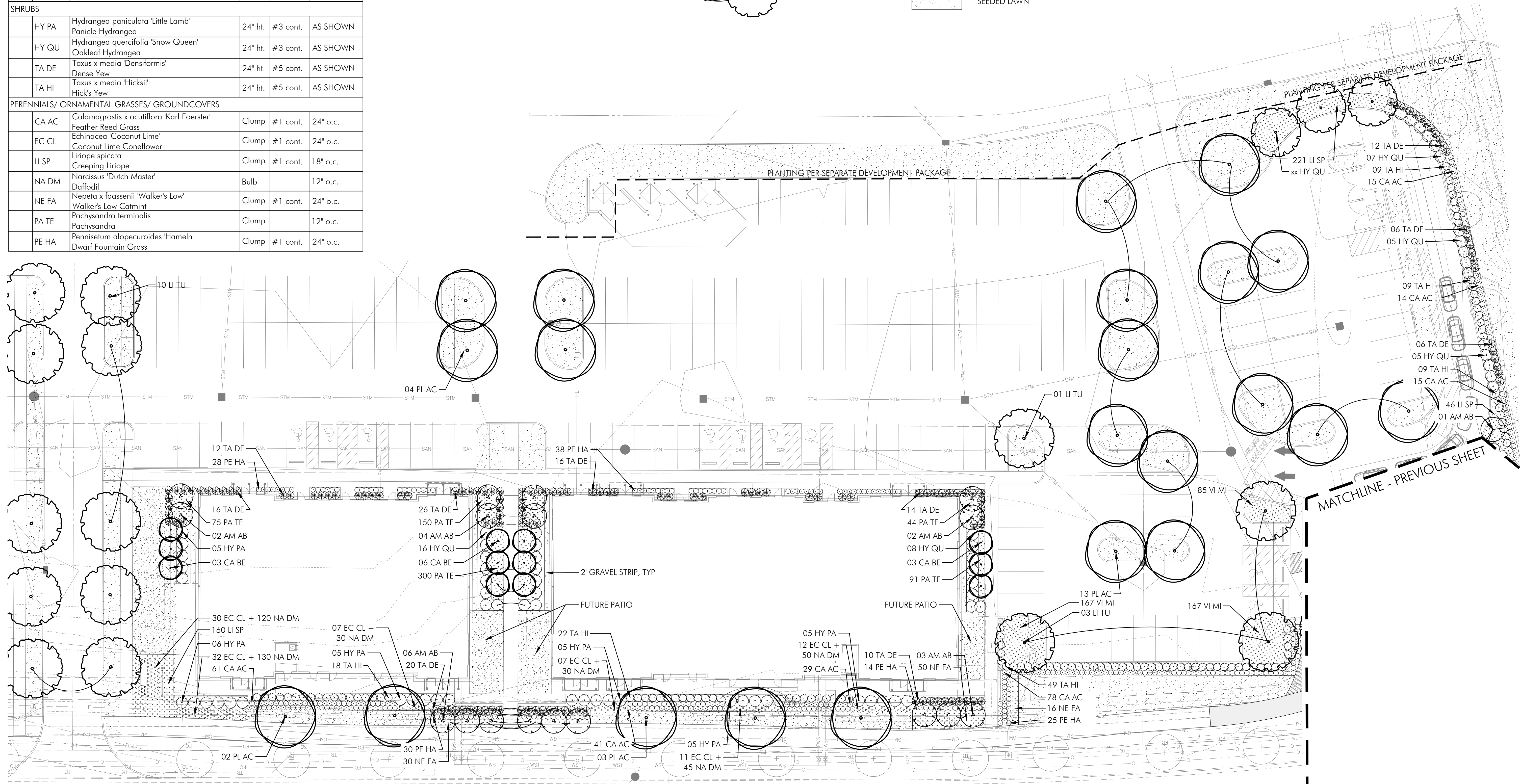
Frontage Planting Plan SCALE: 1" = 20'-0"
