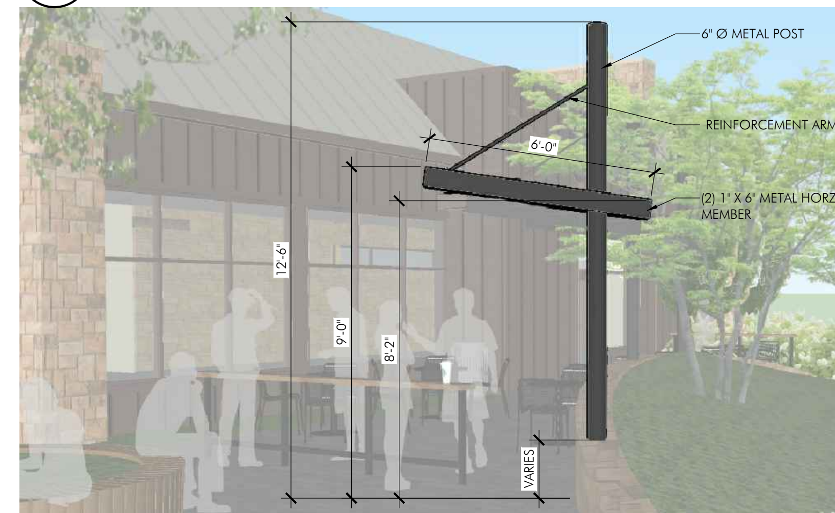
Accent Structure 3/8" = 1'-0"
