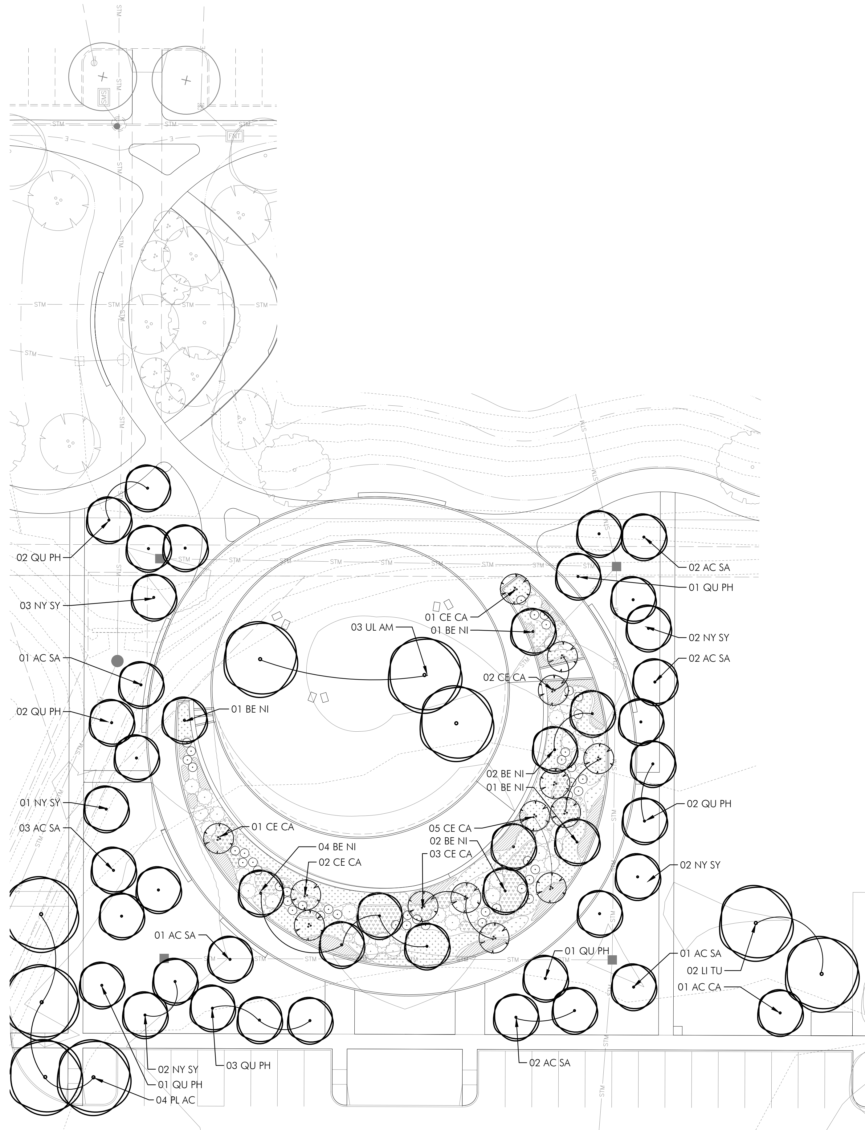
Overlook + Loop Canopy Planting Plan SCALE: 1" = 20'-0"
