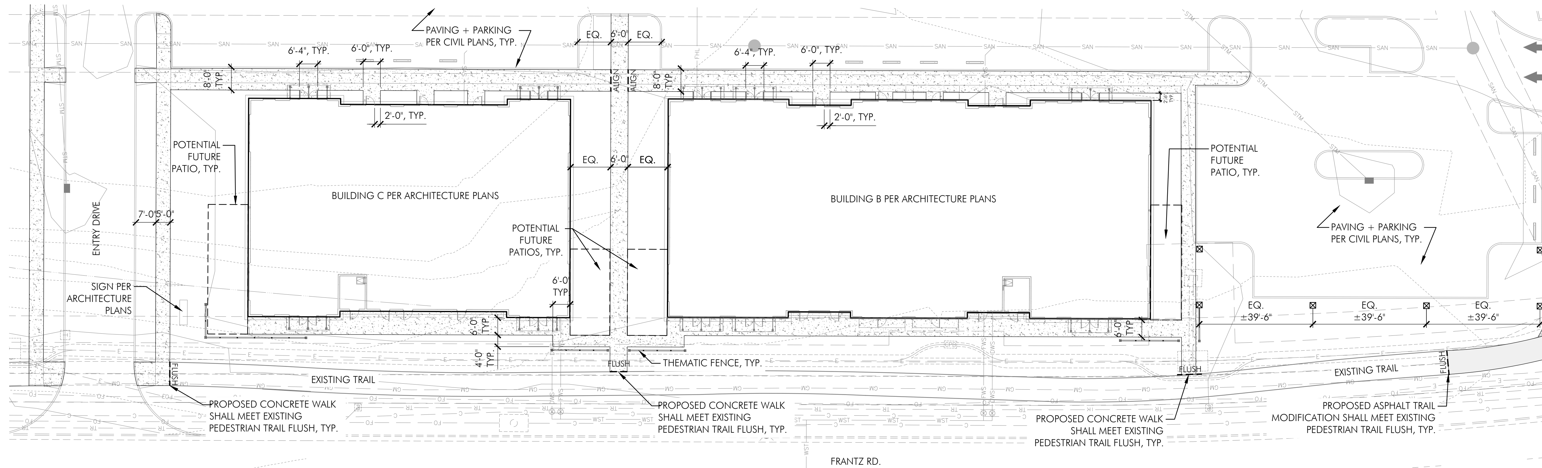
Frontage Layout Plan SCALE: 1" = 20'-0"
