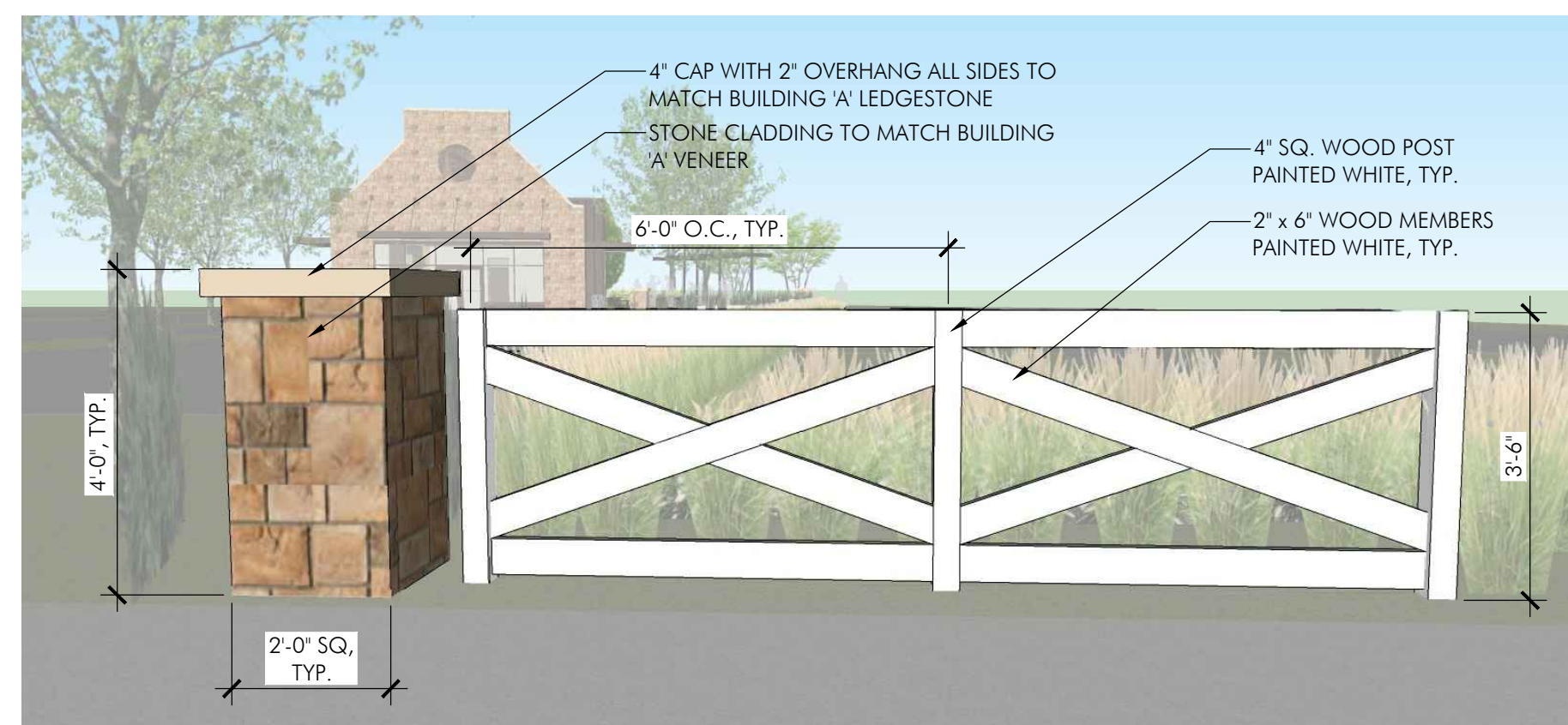
Stone Column & Thematic Fence 1/2" = 1'-0"
