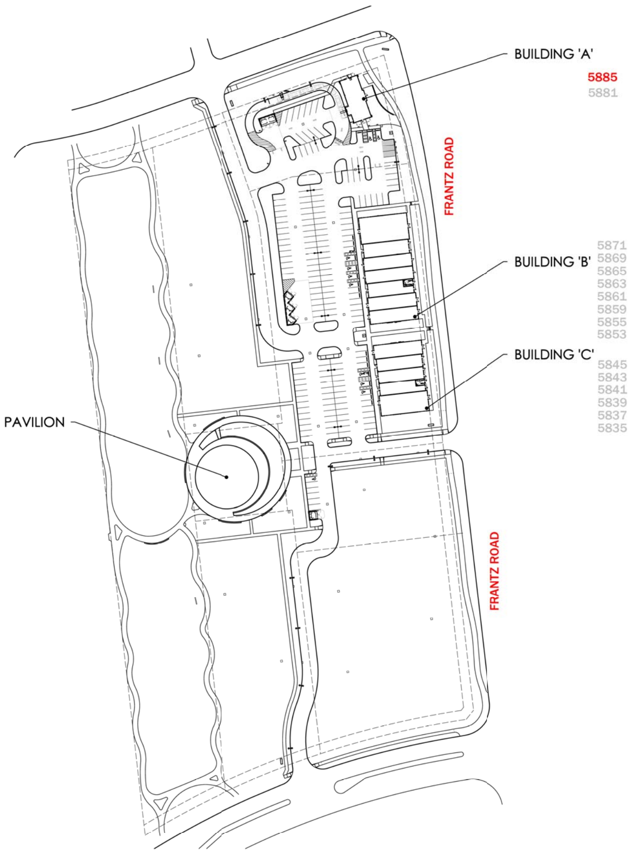
(A) OVERALL SITE DEVELOPMENT PLAN SCALE: 1" = 60'-0"
