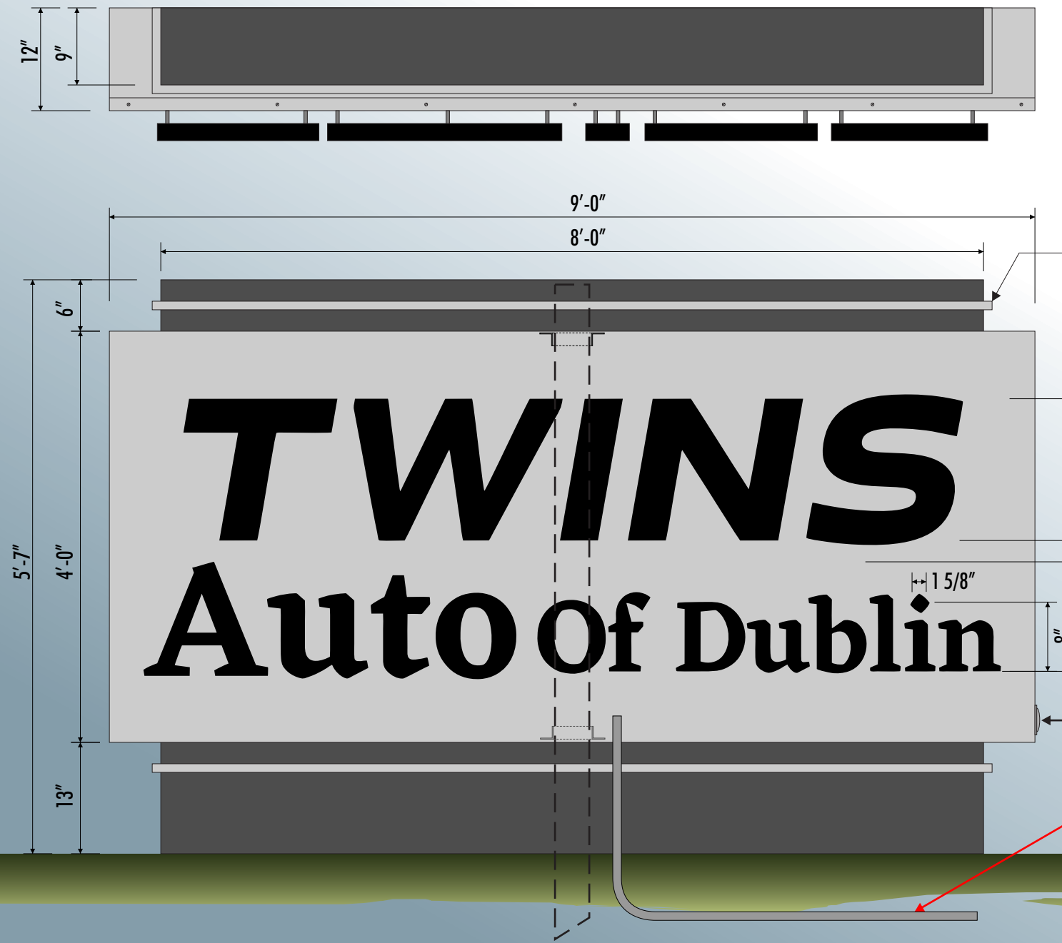
TOP VIEW
