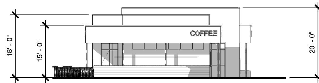
EAST ELEVATION - 1/16" = 1'-0"
