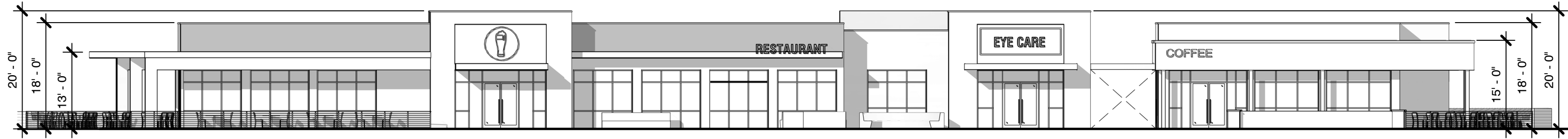
SOUTH ELEVATION - 1/16" = 1'-0"
