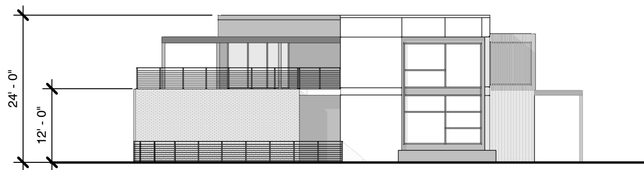
WEST ELEVATION - 1/16" = 1'-0"
