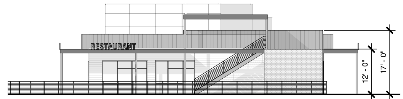
EAST ELEVATION - 1/16" = 1'-0"
