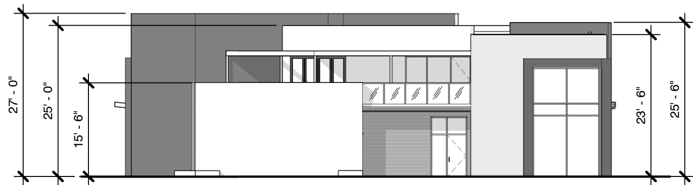
WEST ELEVATION - 1/16" = 1'-0"
