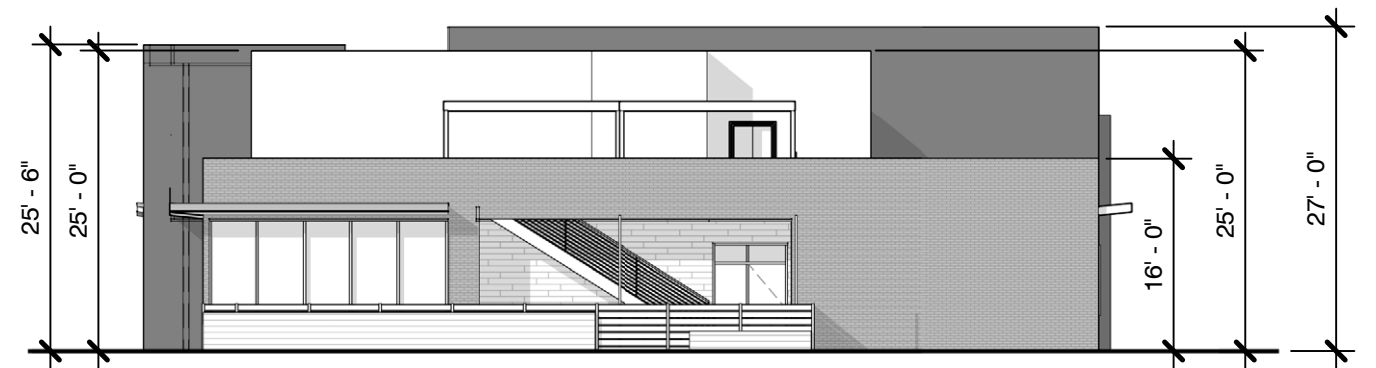
EAST ELEVATION - 1/16" = 1'-0"
