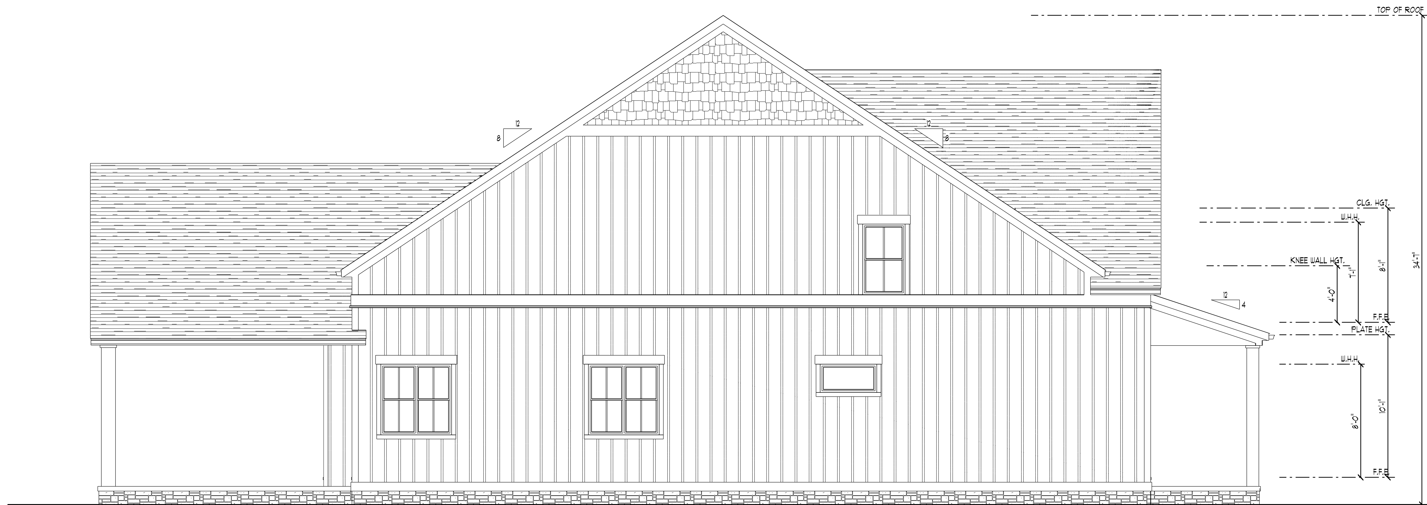
REAR ELEVATION
