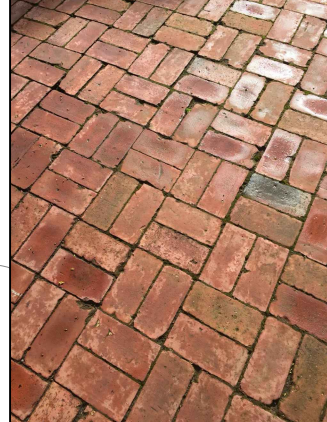
re-purposed clay brick (orange-red) (viable material reused and obtained from site, 4" x 8" x 2-1/4".)
