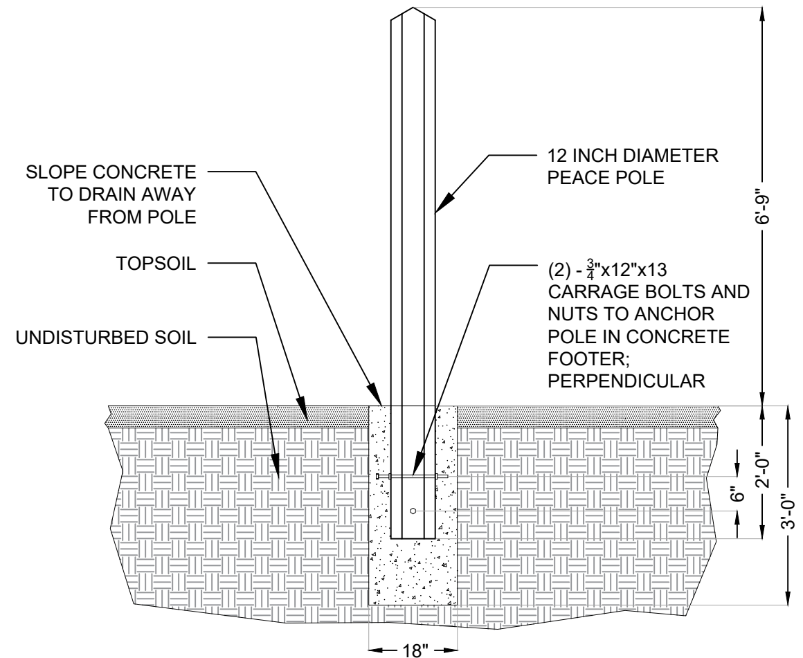
1 PEACE POLE - FOOTING DETAILS L1.0 SCALE :
