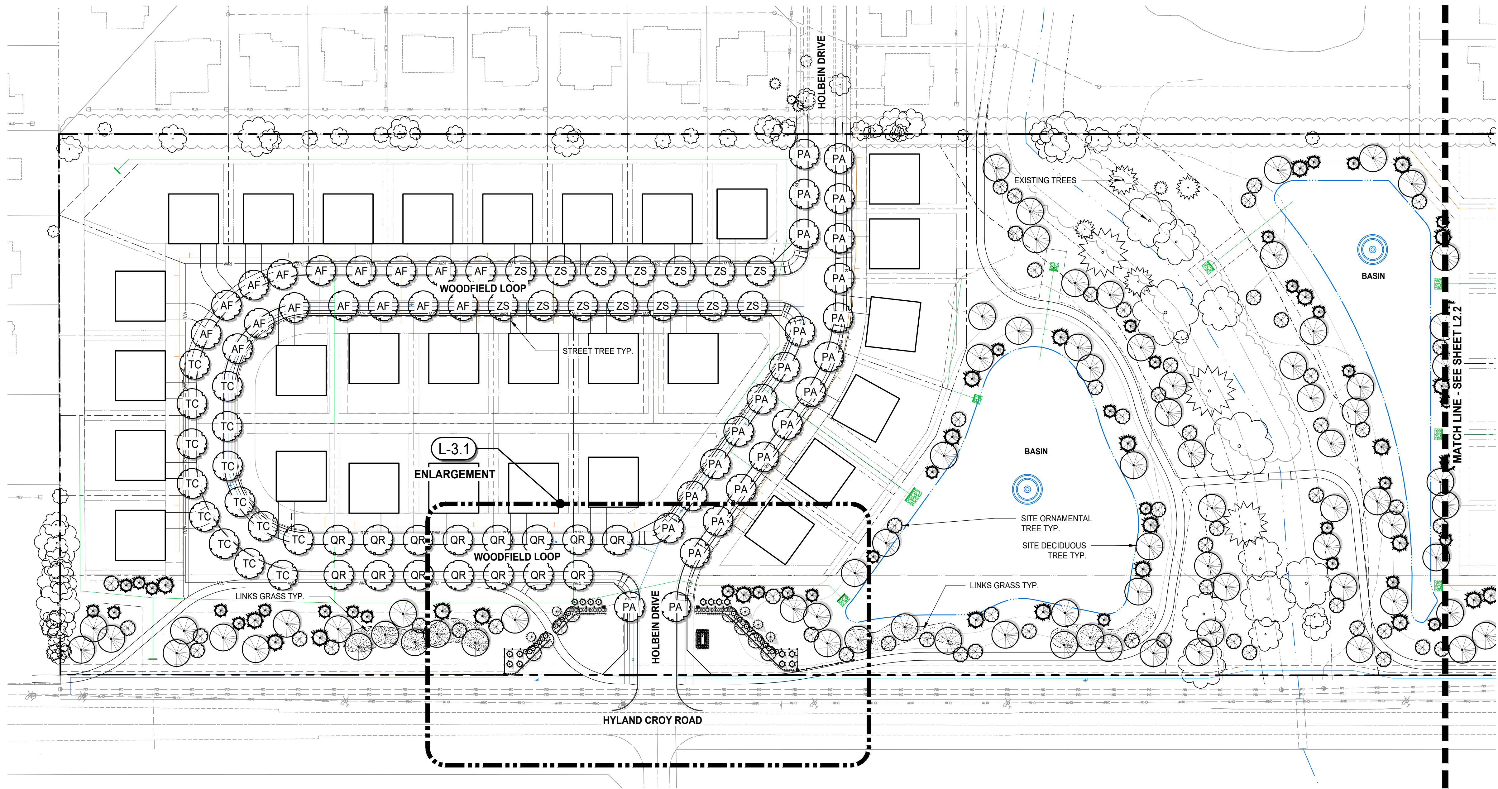
1 SITE LANDSCAPE PLAN Scale: 1" = 60'-0"
