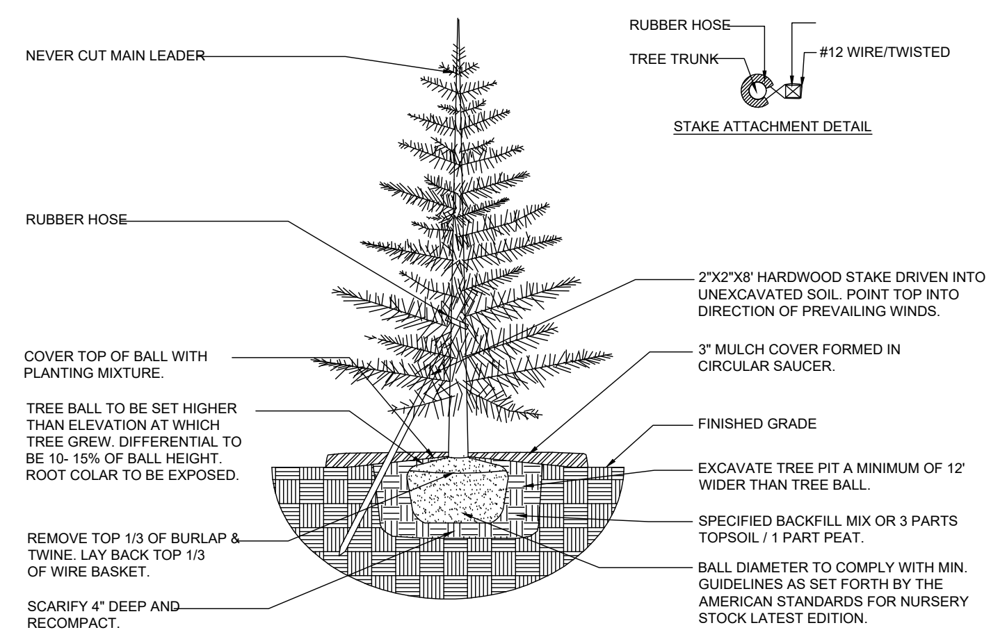
DETAILS: EVERGREEN TREE PLANTING / STAKING Scale: N.T.S TREES UPTO 8' HEIGHT
