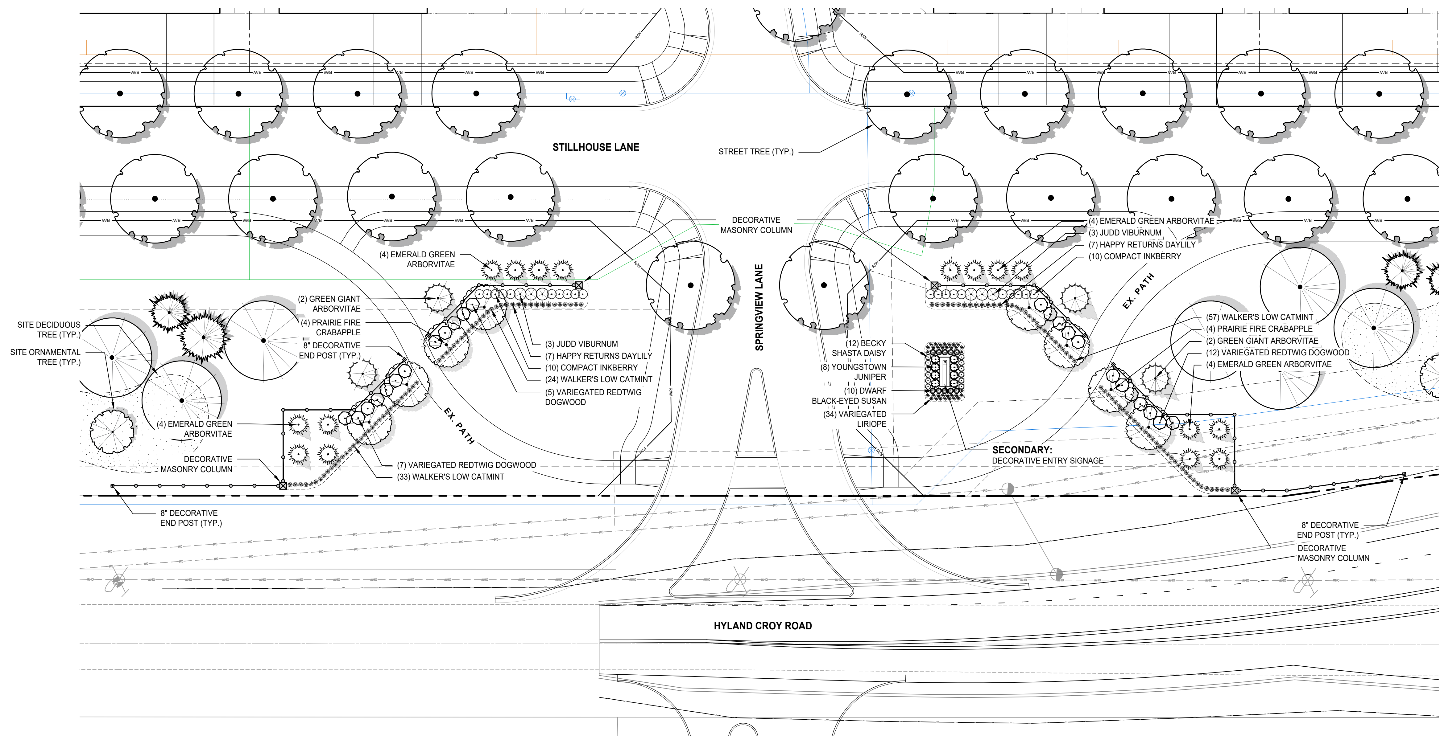
1 SITE LANDSCAPE ENLARGEMENT PLAN Scale: 1" = 20'-0"
