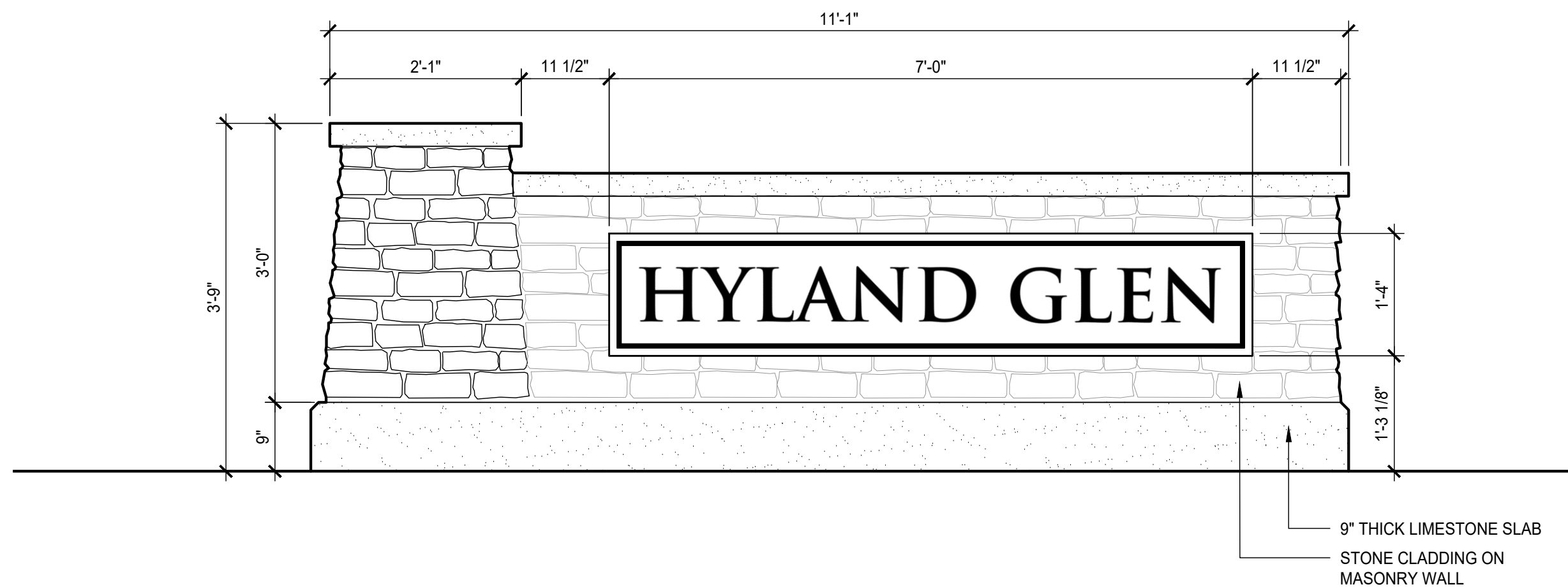
2 SECONDARY ENTRY FEATURE Scale: 3/4" = 1'-0"
