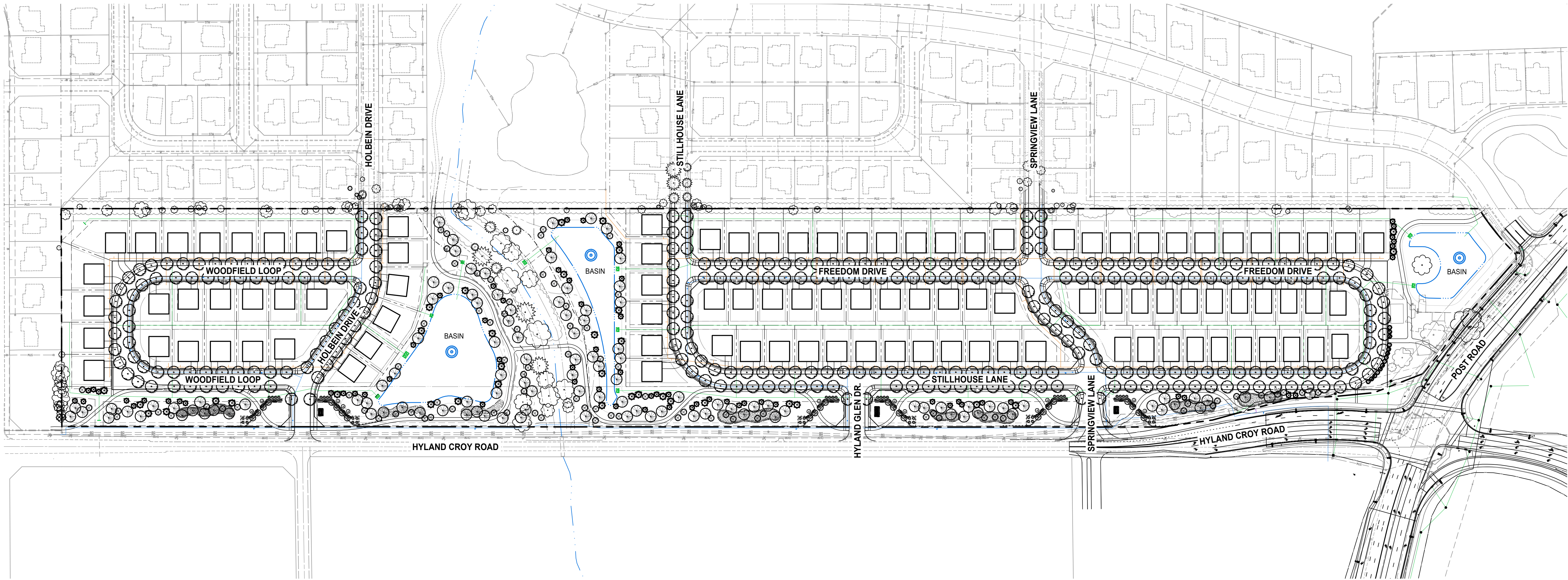
1 TREE REPLACEMENT PLAN NOT TO SCALE
