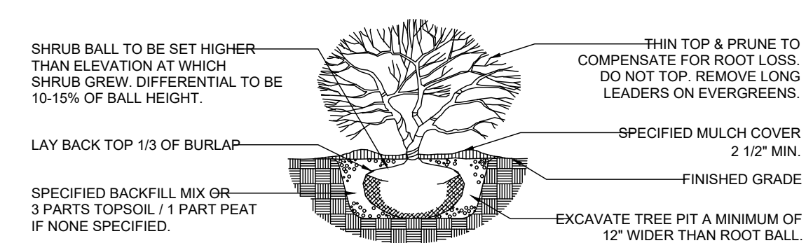
DETAILS: SHRUB TREE PLANTING / STAKING Scale: N.T.S
