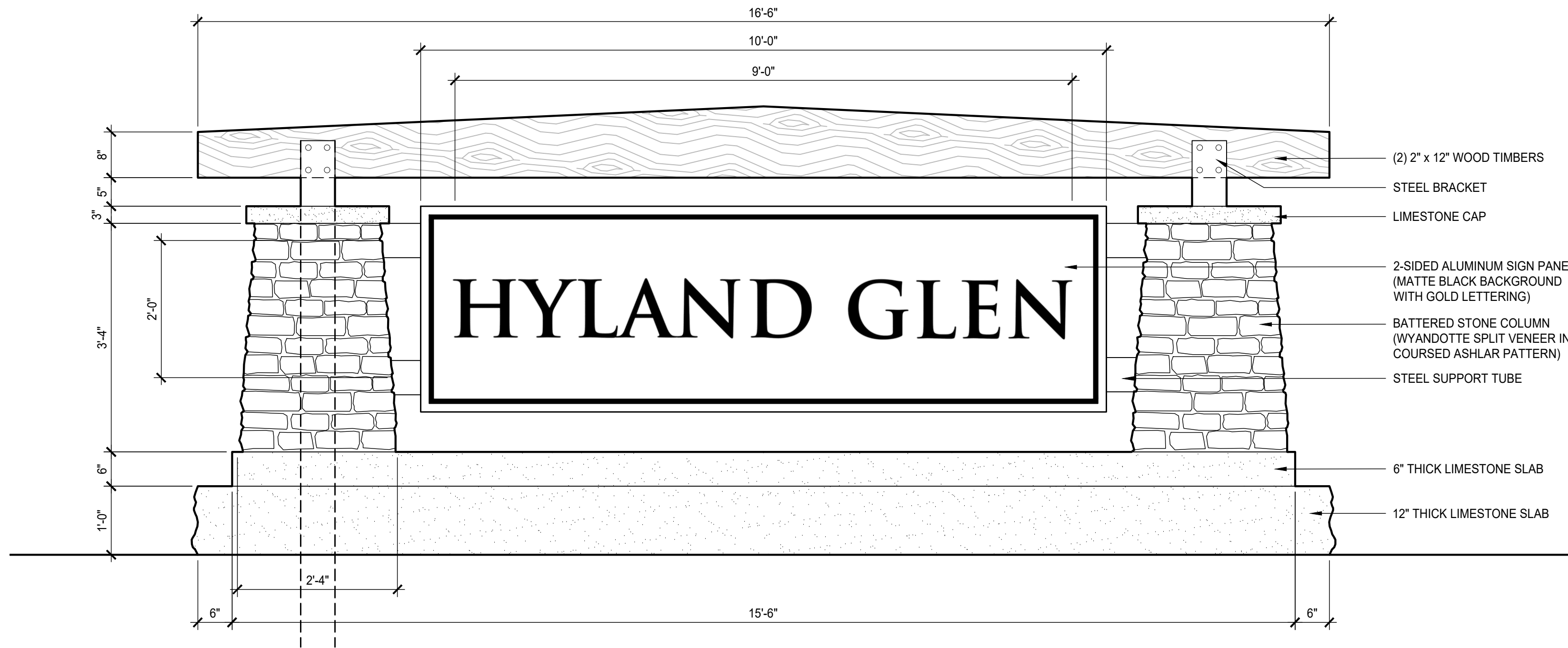
1 PRIMARY ENTRY FEATURE Scale: 3/4" = 1'-0"
