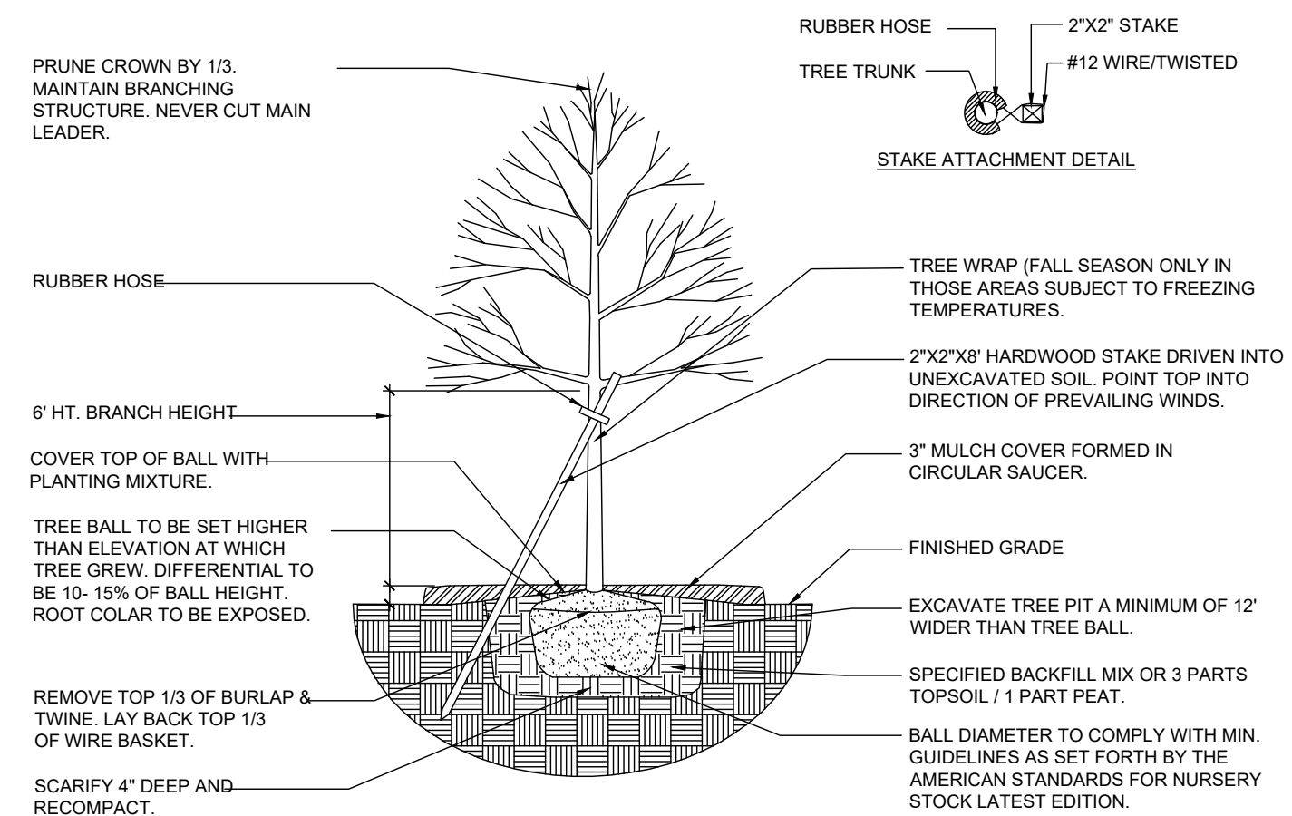
DETAILS: DECIDUOUS TREE PLANTING / STAKING Scale: N.T.S TREES UPTO 3" CALIPER
